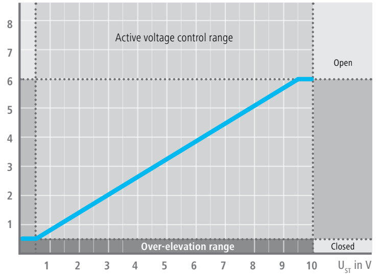
Functional diagram as an example for type MPV 46845-20
